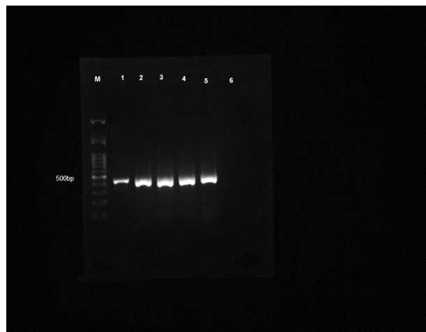
Figure 1. Detection of Cryptosporidium by nested PCR of GP60 gene: M- DNA ladder 100bp, 1-Positive control, 2-Cryptosporidium from suckling BALB/c, 3-Cryptosporidium from suckling rat, 4&5-Cryptosporidium from immunosuppressed rat, 6-Negative control
