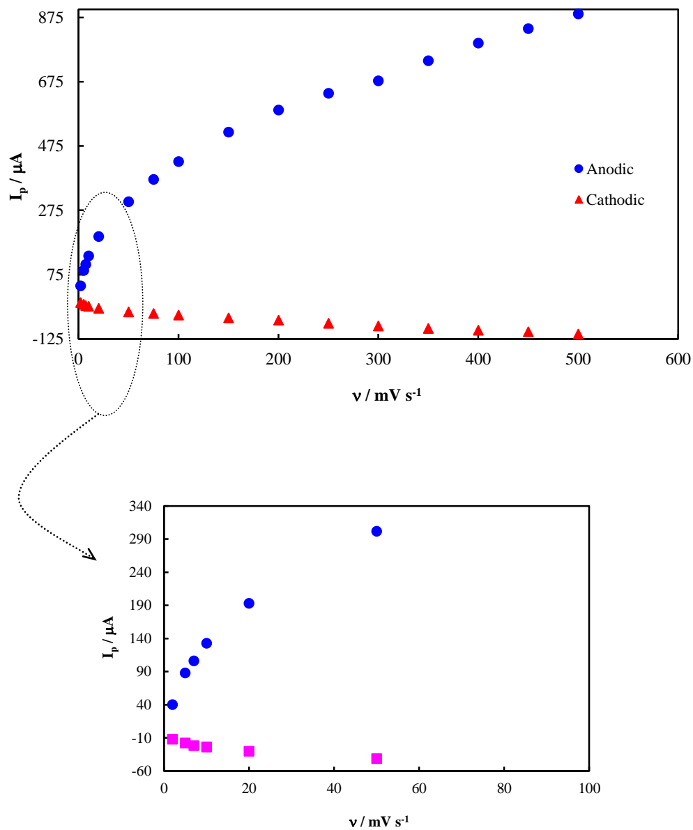
Figure S1. Dependencies of the peak currents on the potential sweep rate. Upper part: main panel; lower part: enlargement of the main panel for small values of the potential sweep rate.
