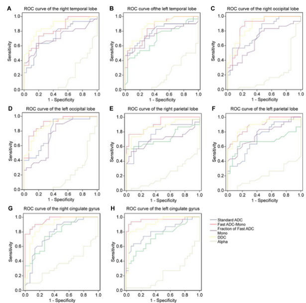
Figure 5. Analyzing the diagnostic efficacy of intravoxel incoherent motion indexes on minimal hepatic encephalopathy through receiver operating characteristic curve analysis. Receiver operating characteristic curves 5A-5H represents the diagnostic efficacy of ADC (blue), D (green), D^* (red), f (purple), DDC (yellow), and \alpha (gray), respectively, for each region of interest of the right temporal lobe, left temporal lobe, right occipital lobe, left occipital lobe, right parietal lobe, left parietal lobe, right cingulate gyrus and left cingulate gyrus.
