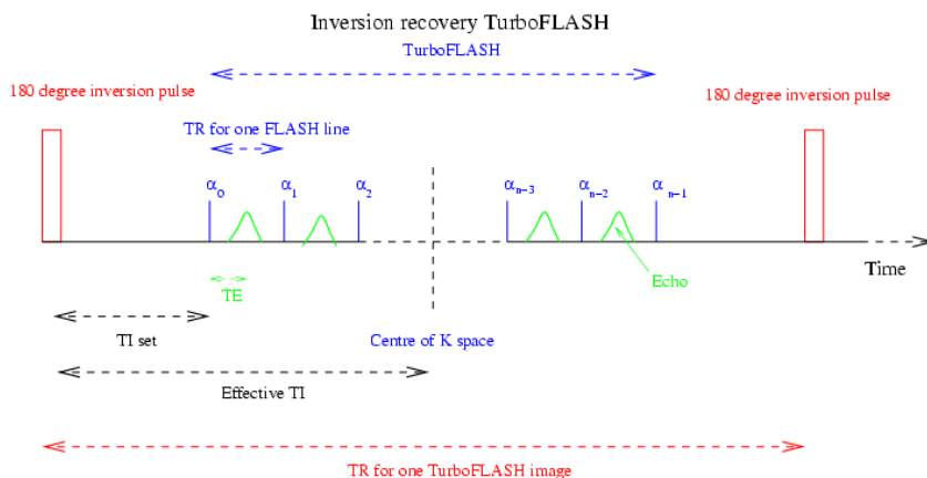
Fig. 1. Inversion recovery gradient-echo TurboFLASH for one image. This is an inversion recovery TurboFLASH with n α pulses, where the n/2th line traverses the centre of K space (for Linear Phase-Encoding). "TI set" is the time between 180° inversion pulse and the first α excitation pulse. The effective TI is the time from the inversion pulse to the mid line of K space (n/2th). TE and TR are the echo time and repetition time respectively. Imaging gradients are not shown in this diagram.
