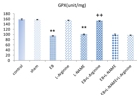
Figure 2. The effect of ethidium bromide, L-arginine and L-NAME injection alone and in combination on the left side of the CA1 hippocampus on glutathione peroxidase in male rats
