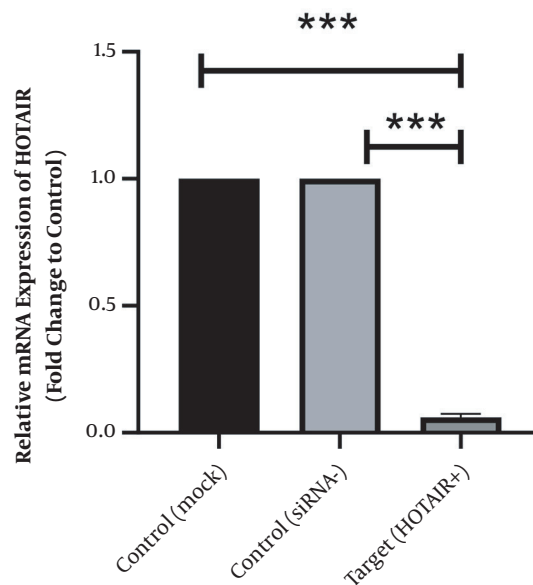
Figure 1. Effects of HOTAIR specific siRNA on suppressing HOTAIR transcript after treatment with 50 ng siRNA after 48 hours of treatment. Data expressed as mean \pm standard deviation (the stars *** show the P-value less than 0.001 compared to the control group).
