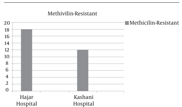
Figure 1. Prevalence of Methicillin-Resistant Staphylococcus aureus in Each Hospital
