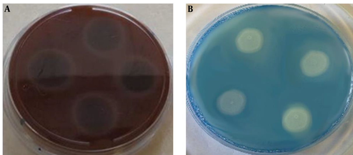
Figure 2. Translucent (clear) zone around the colony for (A) hemolysin and (B) proteinase activity
