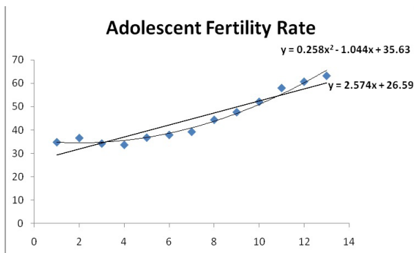
Figure 1. Comparison of Linear and Quadratic Trendlines for Adolescent Fertility Rate (AFR)
