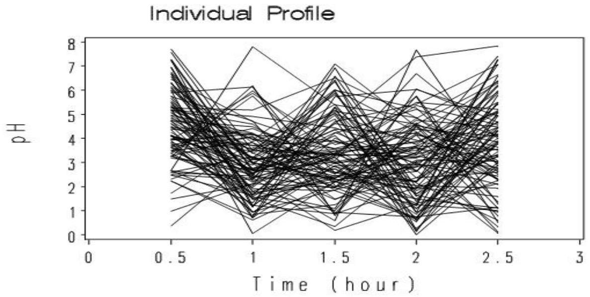
Figure 1, Individual profiles of pH level over time.
