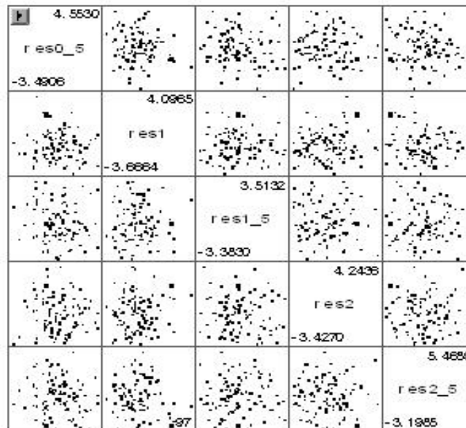
Figure 4: Correlation structure of OLS residual over time
