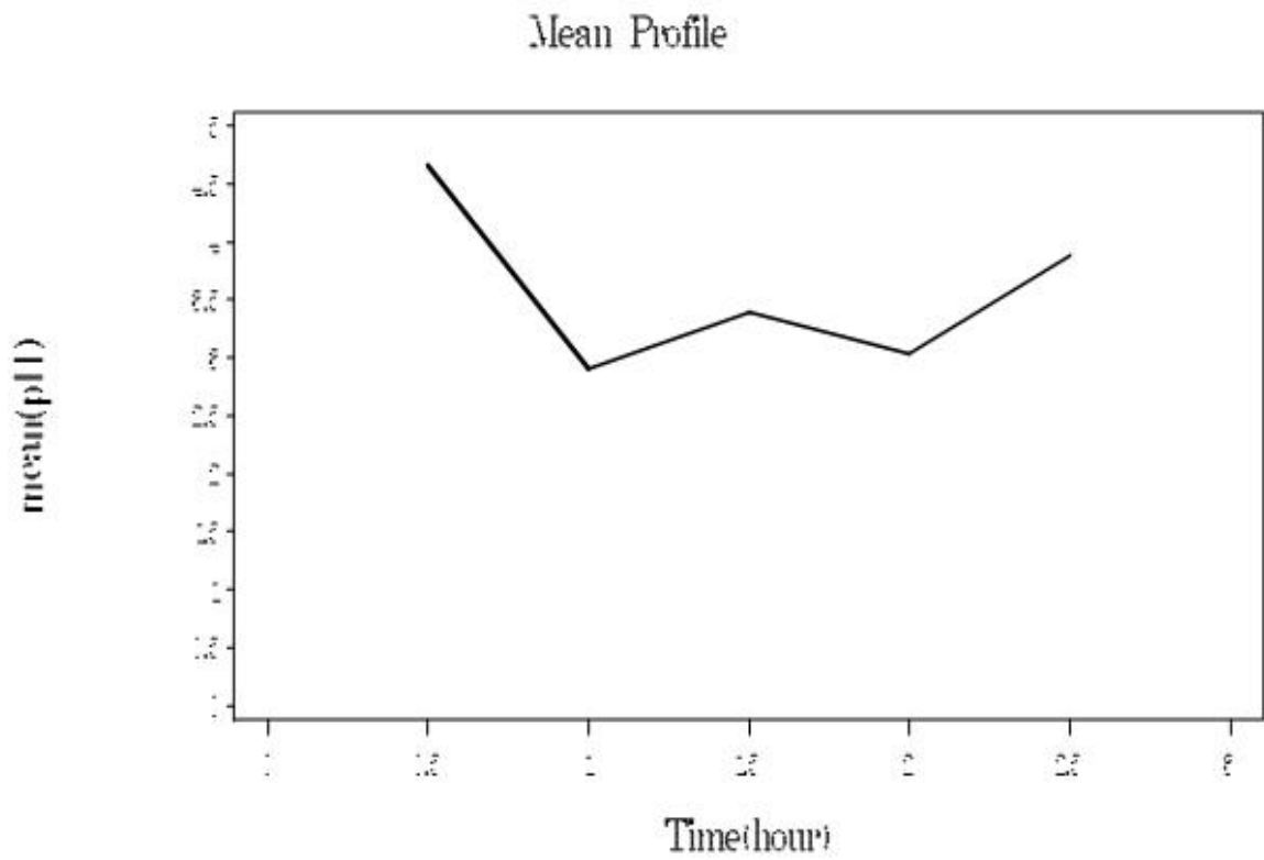
Figure 2: Mean profile of pH level over time
