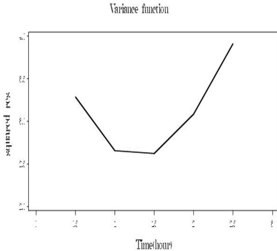
Figure 3: Variance profile of pH level over time.
