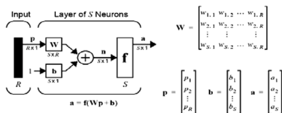
Figure 2. MLP Neural Network [Matlab® Help]
