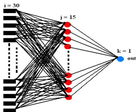
Figure 3. Proposed Neural Network (NN) Adapted From [34]
