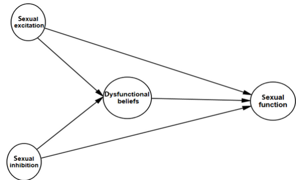
Figure 1. The hypothetical research model
