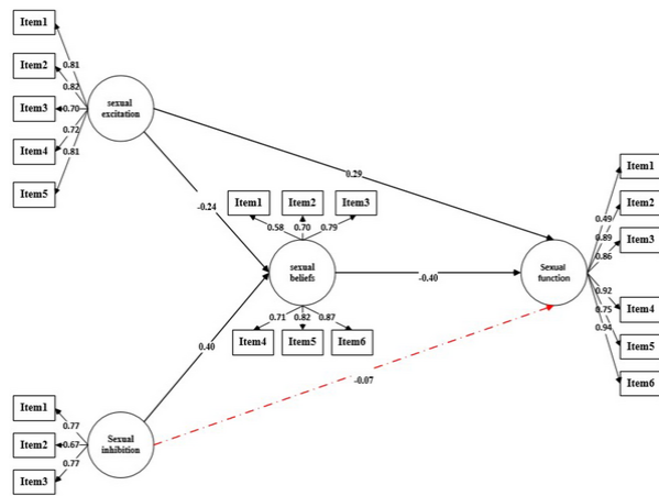
Figure 2. The structural model of the research
