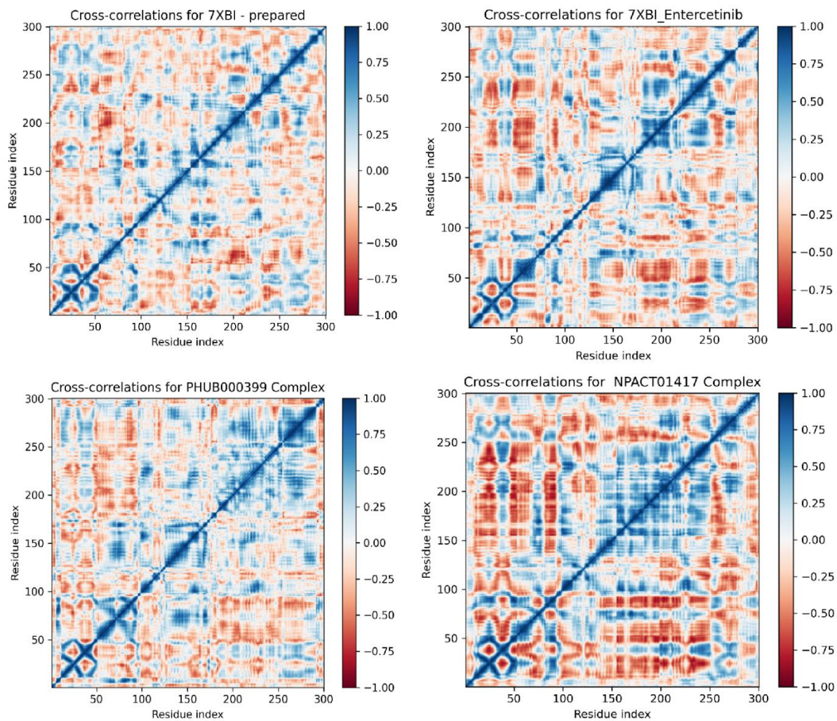
Figure S1. Dynamic cross-correlation analysis (DCCM) results. A TrkA-co-crystal ligand complex B) TrkA-Entrectinib complex, C TrkA-PHUB000399 complex and D TrkA-NPACT01417 complex.
