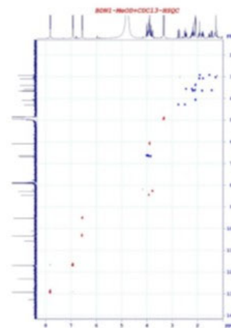
Figure S5. HSQC spectrum of compound 1
