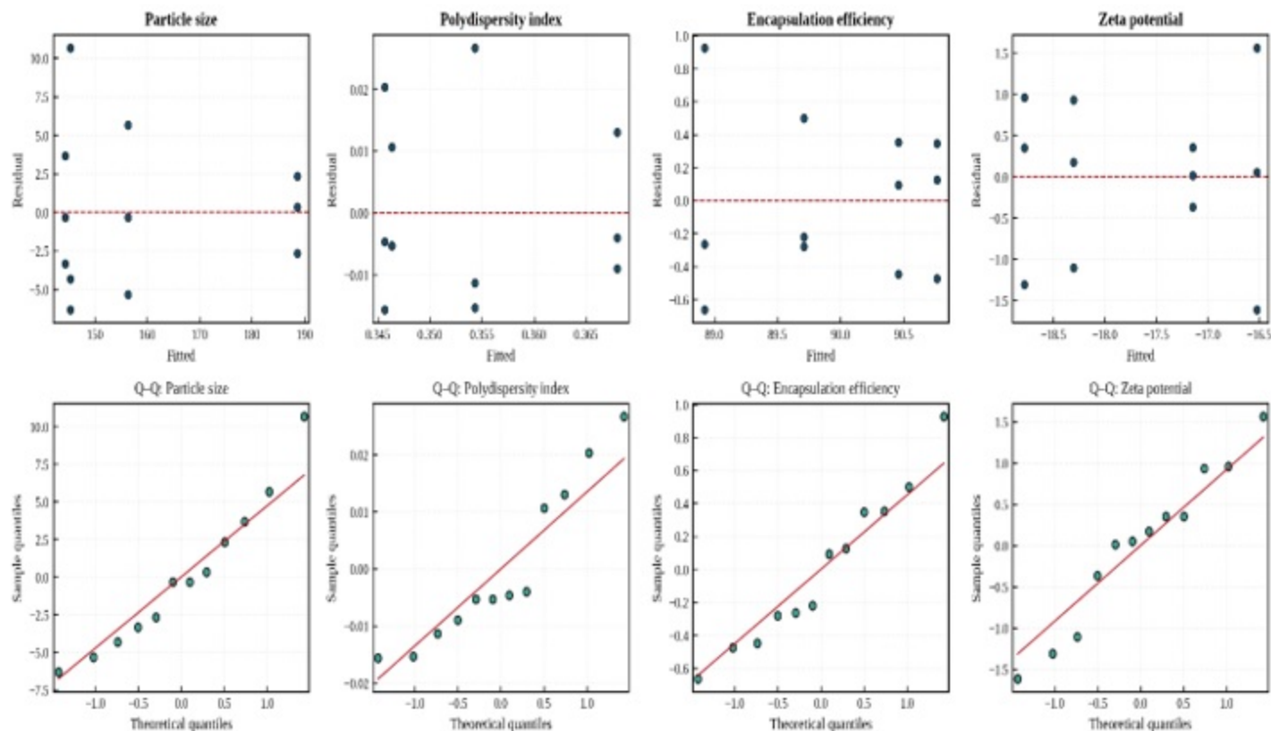
Supplementary Figure S2. Residual-versus-fitted (top) and normal Q-Q (bottom) plots for the four coded factorial models
